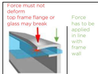
Figure 1a: Clamp Force Locations
