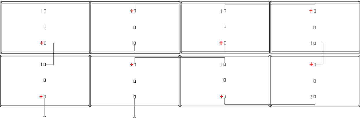
Landscape Stringing
