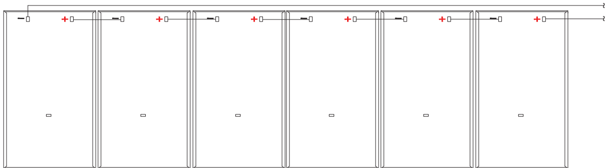
LeapFrog (Portrait Stringing)
