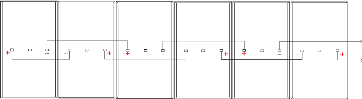
Landscape Stringing
