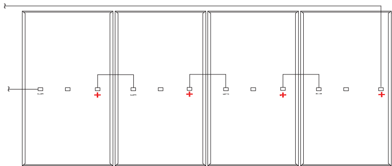
Leapfrog Stringing (Portrait)
