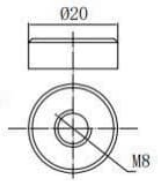
Terminal Dimensions
