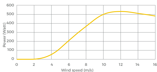
POWER CURVE
