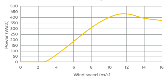
POWER CURVE
