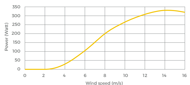
POWER CURVE
