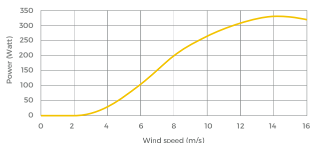
POWER CURVE
